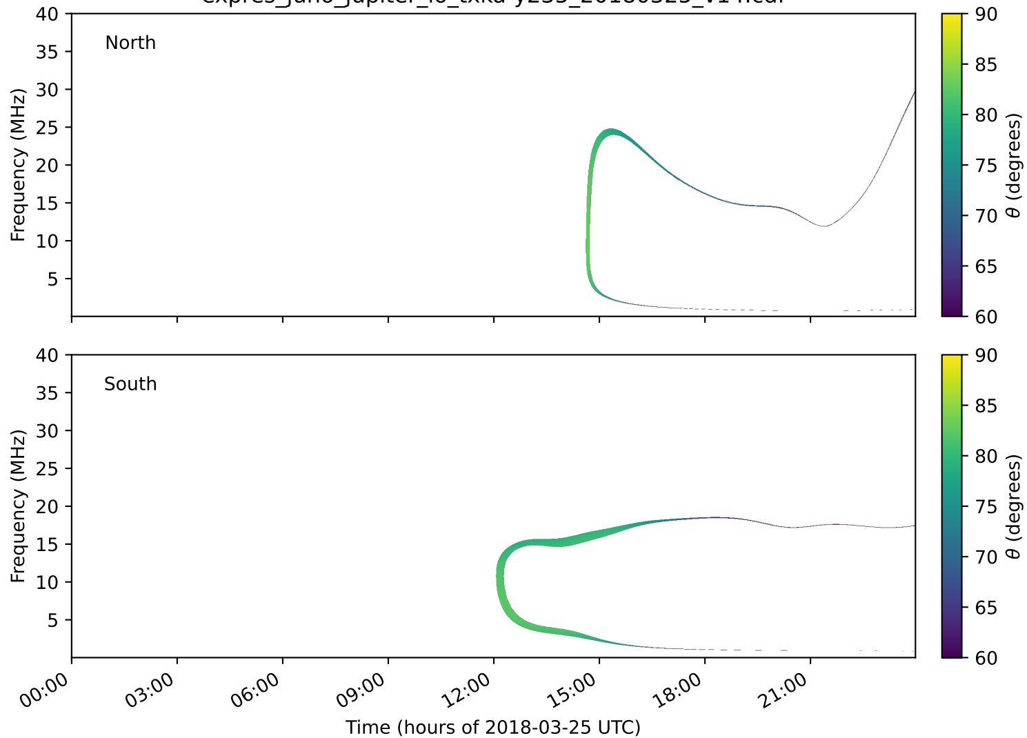
expres_juno_jupiter_io_txka-y235_20180325_v14.cdf
