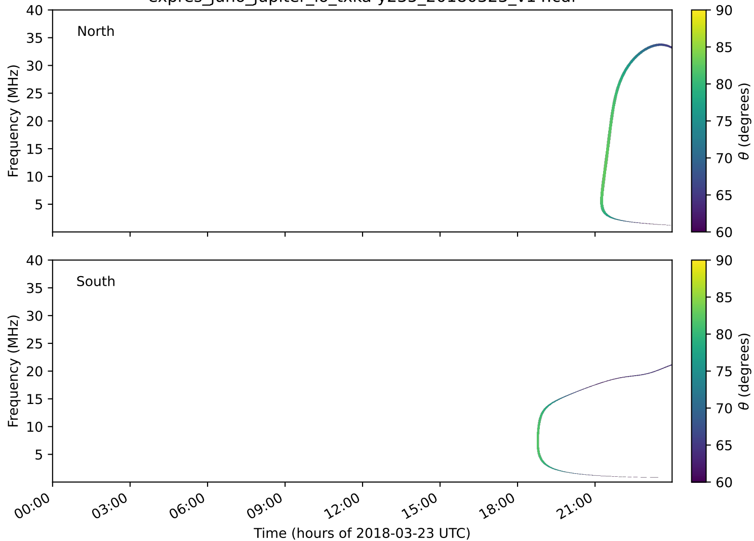
expres_juno_jupiter_io_txka-y235_20180323_v14.cdf
