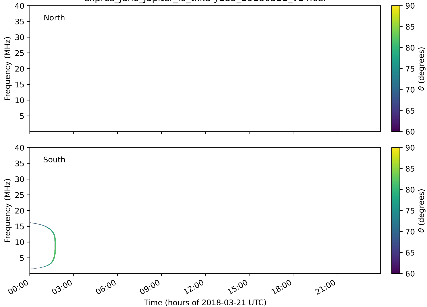
expres_juno_jupiter_io_txka-y235_20180321_v14.cdf
