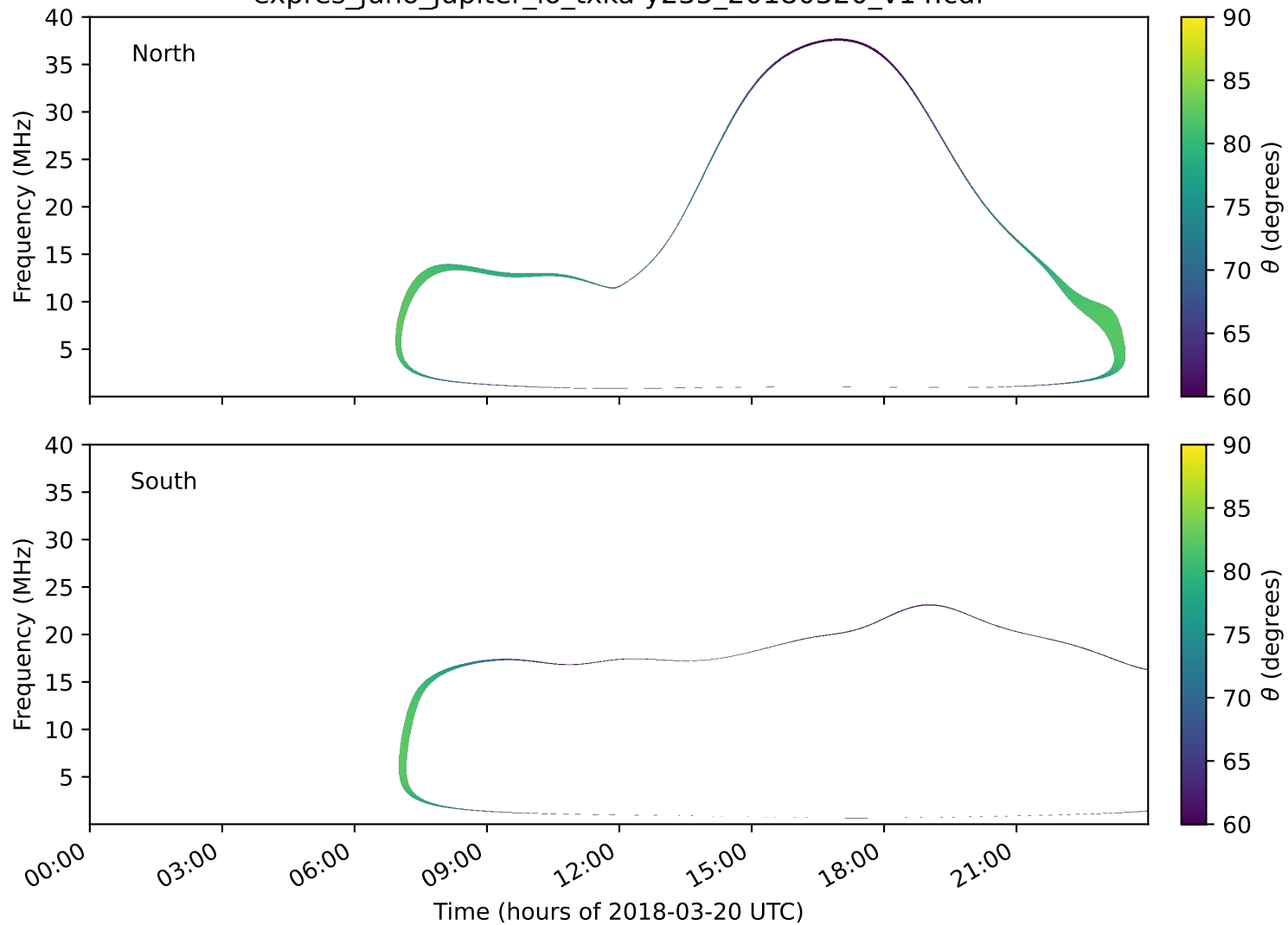
expres_juno_jupiter_io_txka-y235_20180320_v14.cdf
