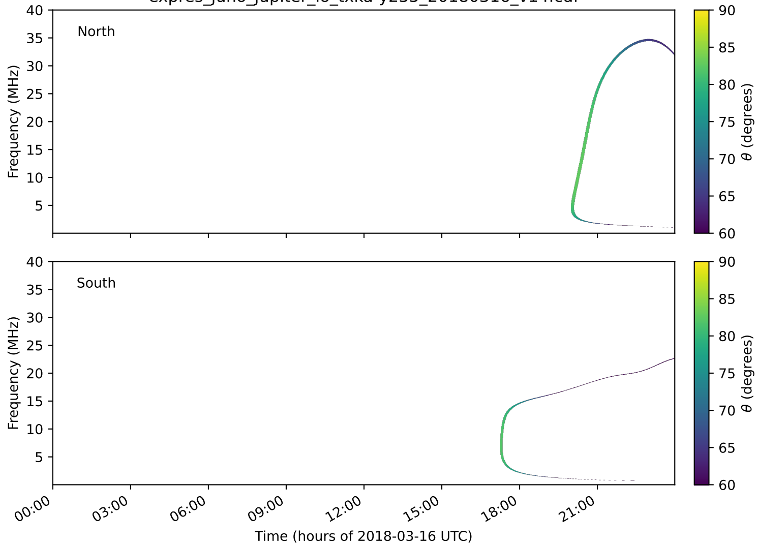
expres_juno_jupiter_io_txka-y235_20180316_v14.cdf
