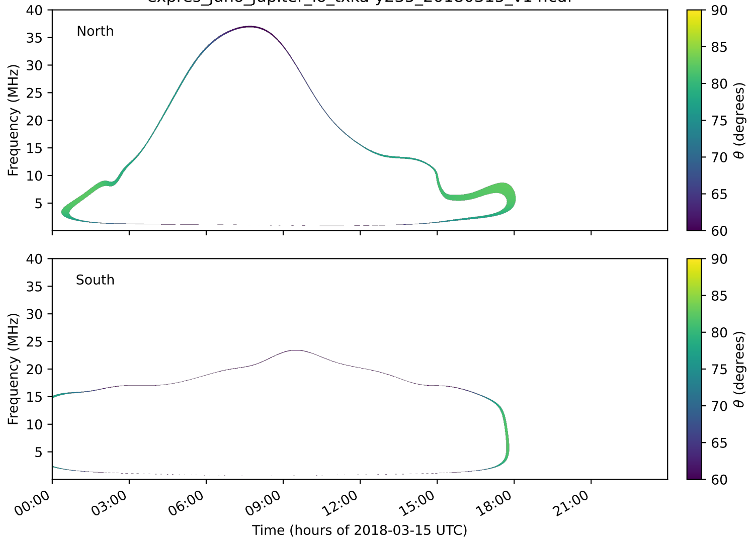
expres_juno_jupiter_io_txka-y235_20180315_v14.cdf
