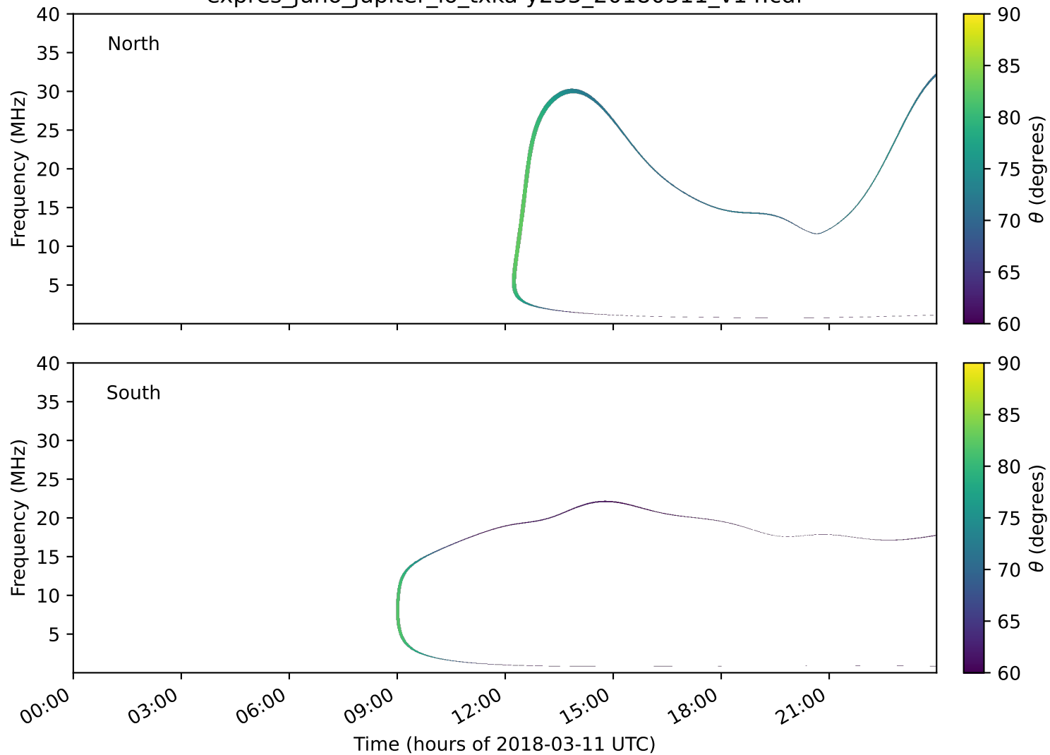
expres_juno_jupiter_io_txka-y235_20180311_v14.cdf
