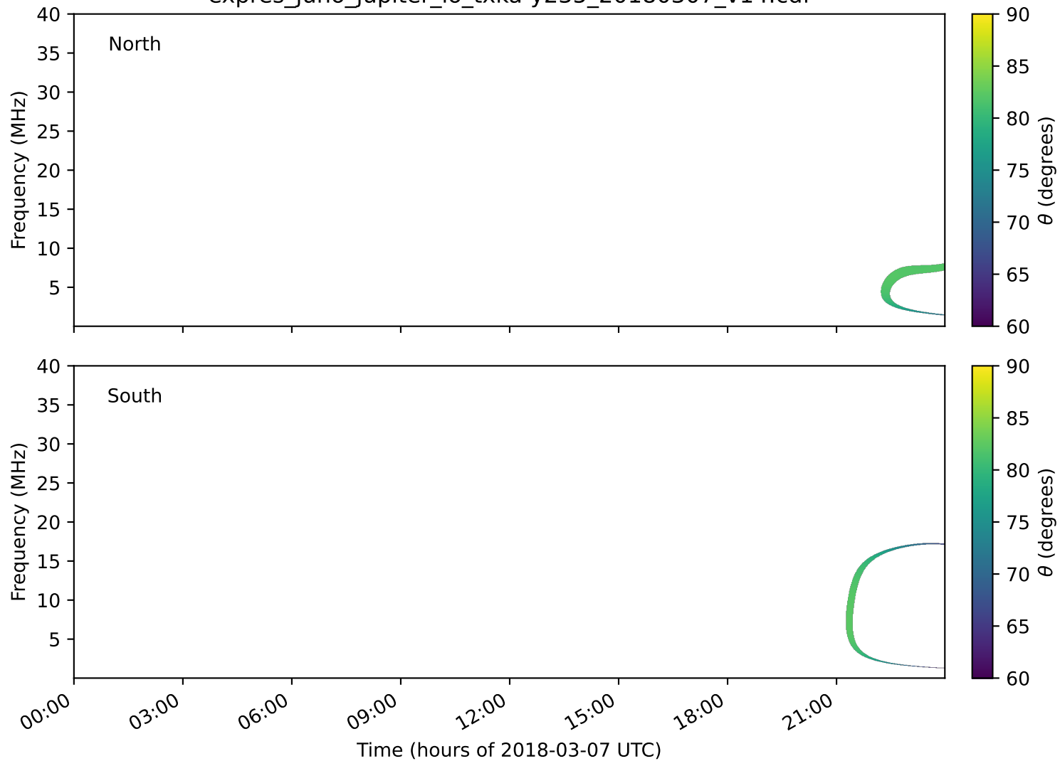
expres_juno_jupiter_io_txka-y235_20180307_v14.cdf
