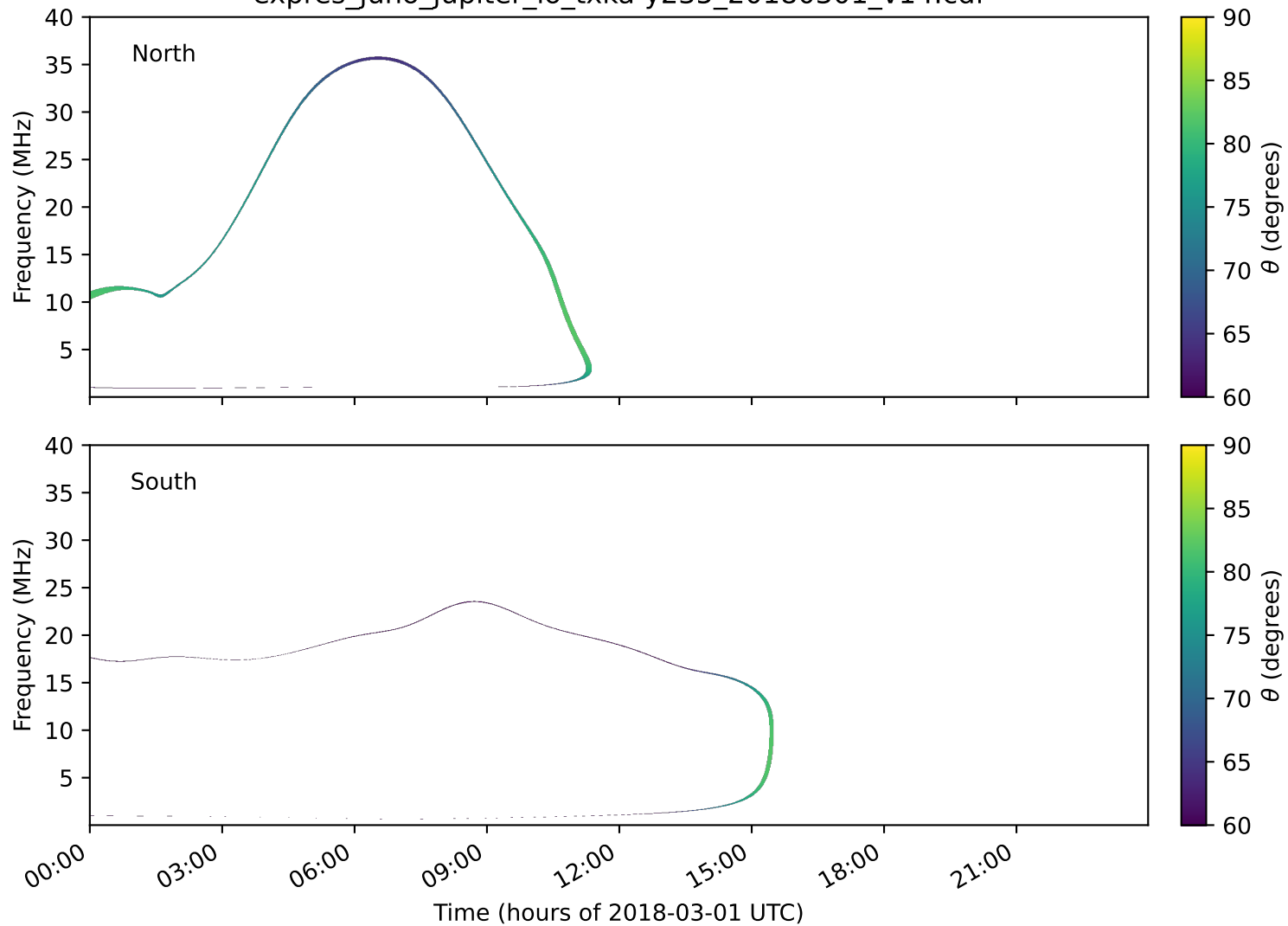
expres_juno_jupiter_io_txka-y235_20180301_v14.cdf
