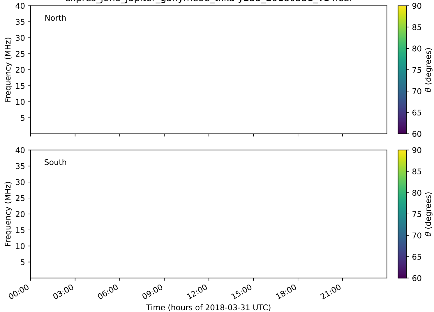
expres_juno_jupiter_ganymede_txka-y235_20180331_v14.cdf
