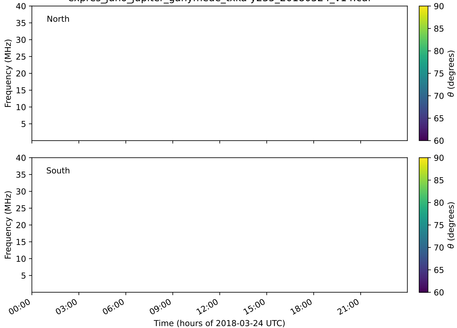
expres_juno_jupiter_ganymede_txka-y235_20180324_v14.cdf
