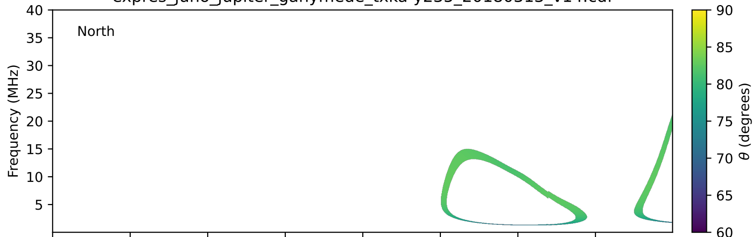
expres_juno_jupiter_ganymede_txka-y235_20180313_v14.cdf
