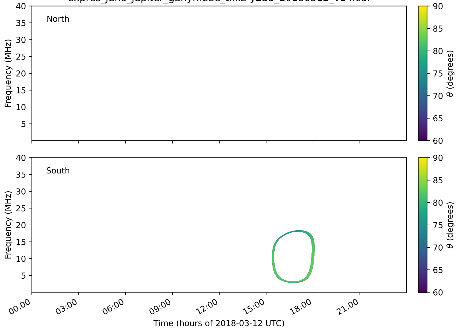
expres_juno_jupiter_ganymede_txka-y235_20180312_v14.cdf
