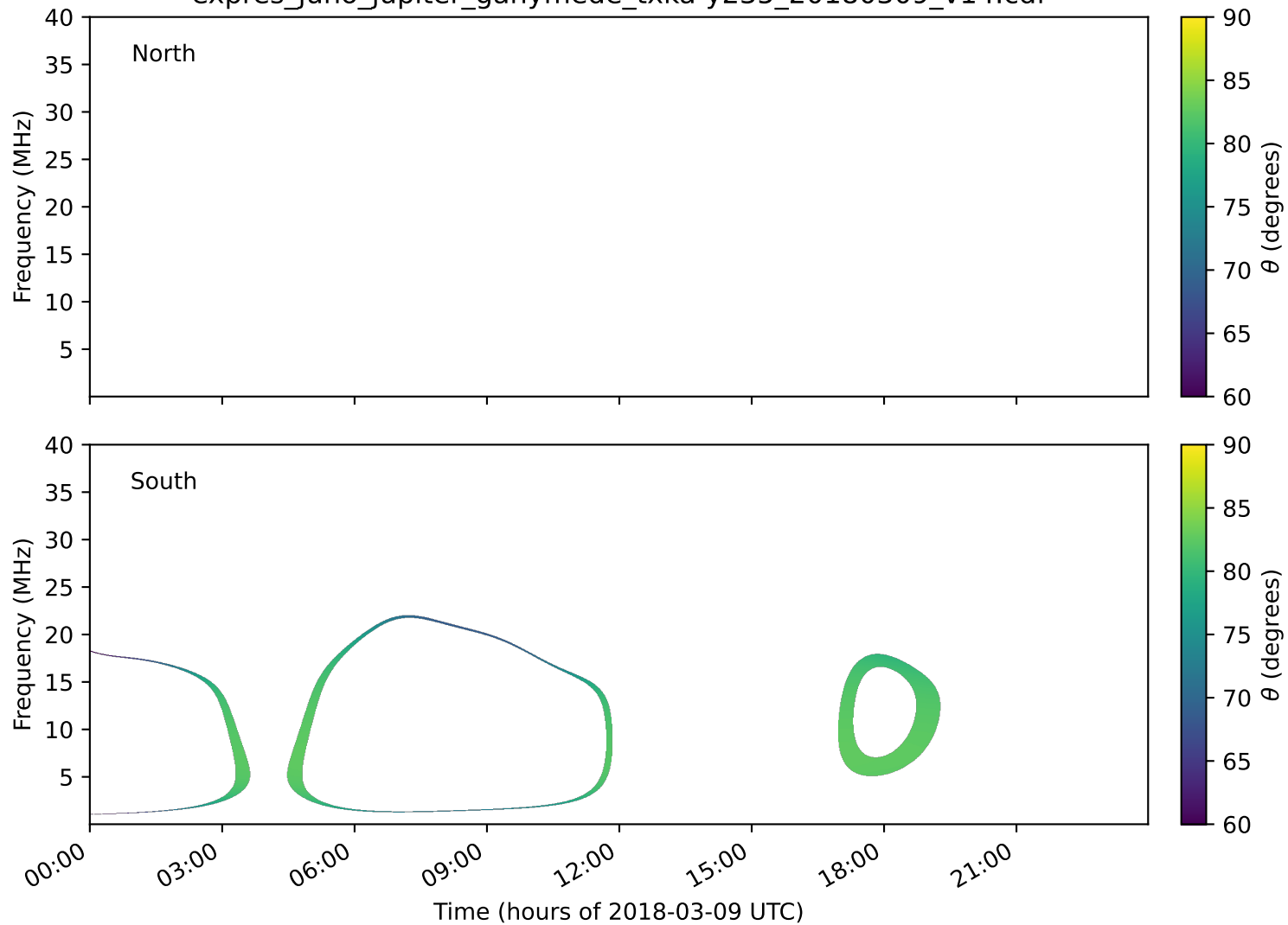
expres_juno_jupiter_ganymede_txka-y235_20180309_v14.cdf
