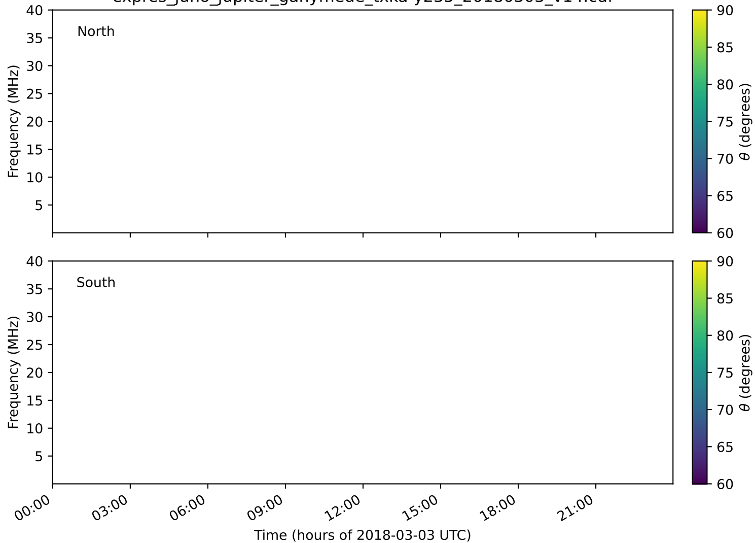
expres_juno_jupiter_ganymede_txka-y235_20180303_v14.cdf
