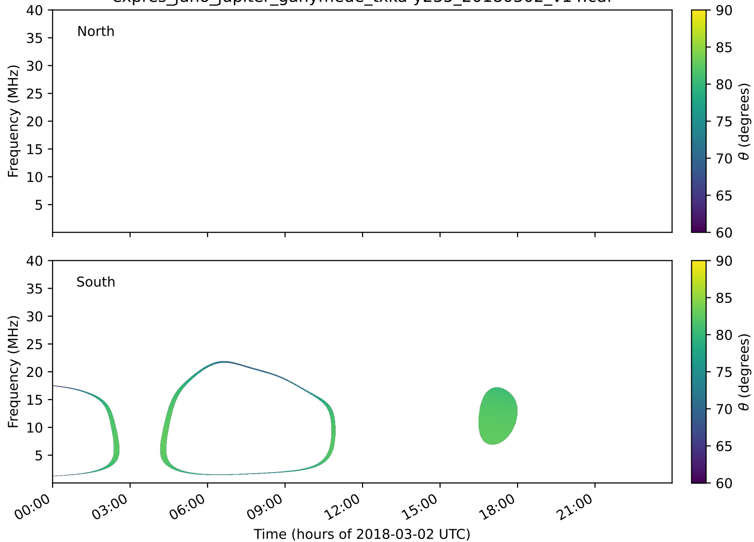
expres_juno_jupiter_ganymede_txka-y235_20180302_v14.cdf
