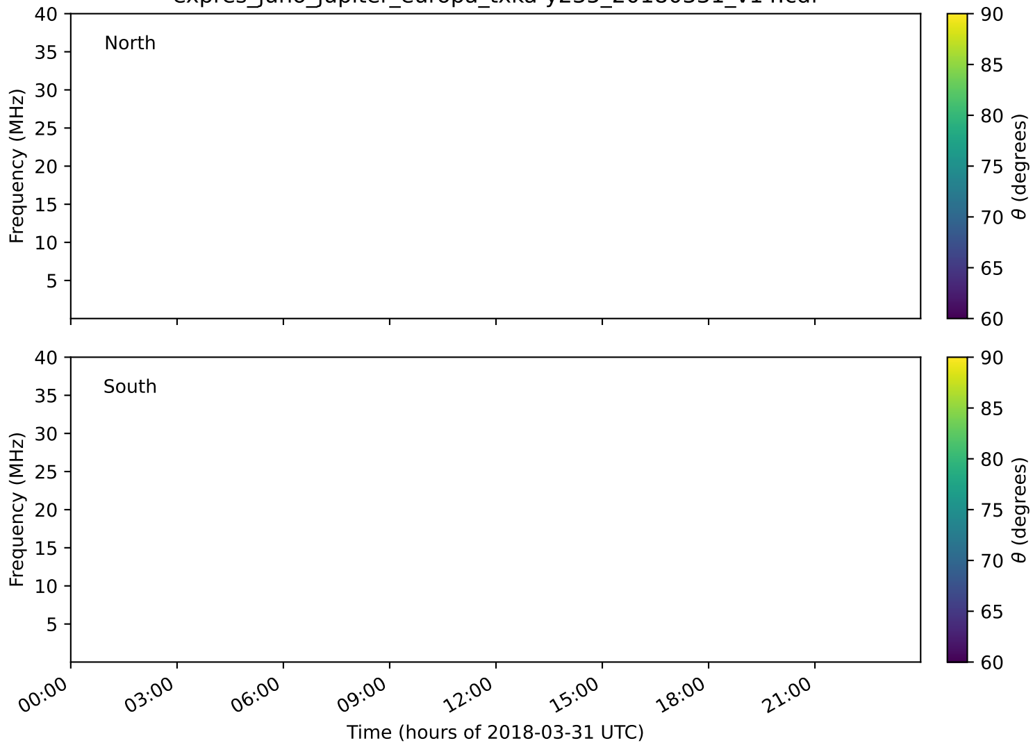
expres_juno_jupiter_europa_txka-y235_20180331_v14.cdf
