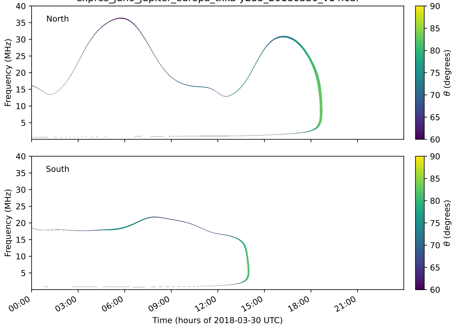
expres_juno_jupiter_europa_txka-y235_20180330_v14.cdf
