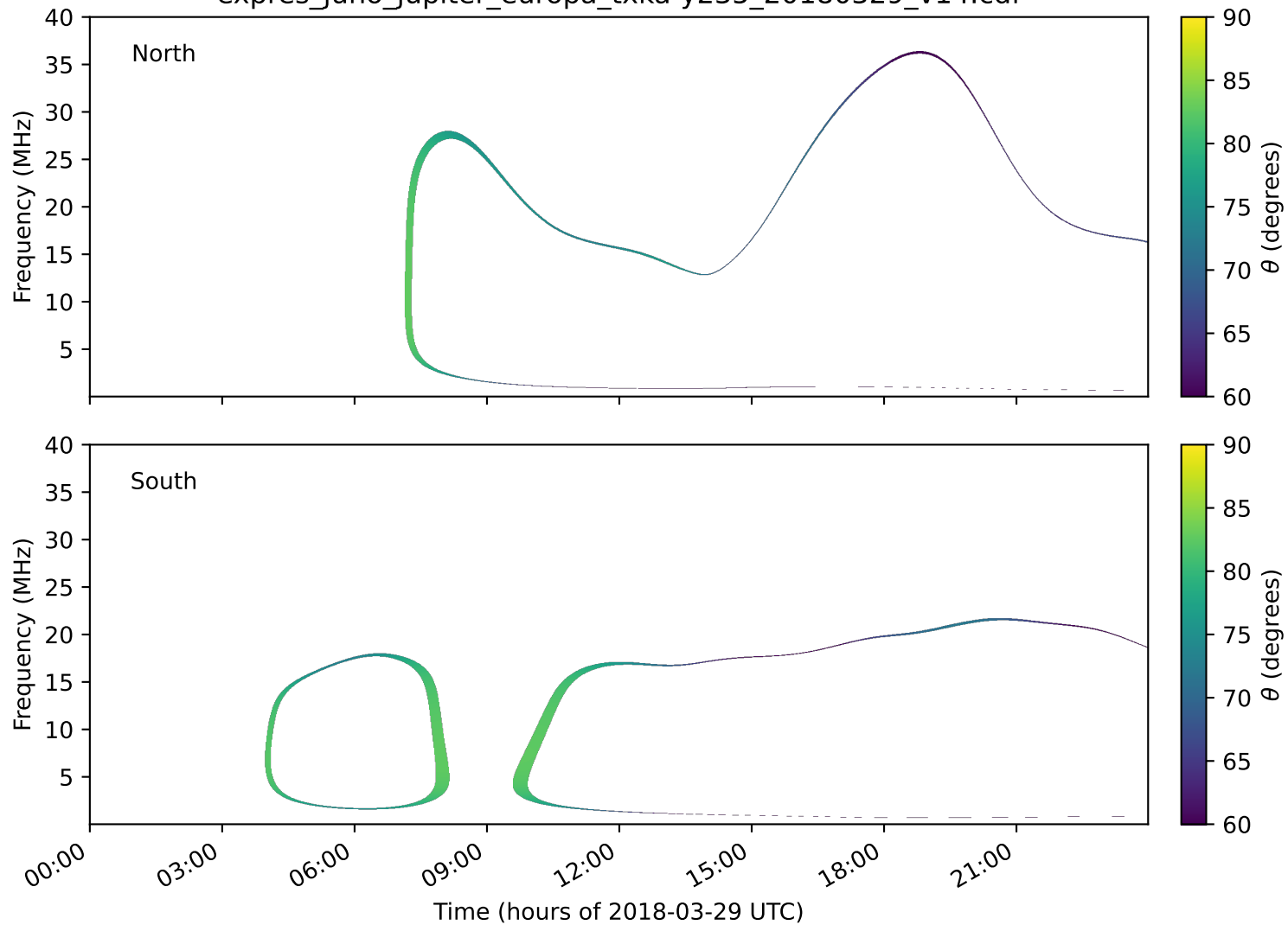
expres_juno_jupiter_europa_txka-y235_20180329_v14.cdf
