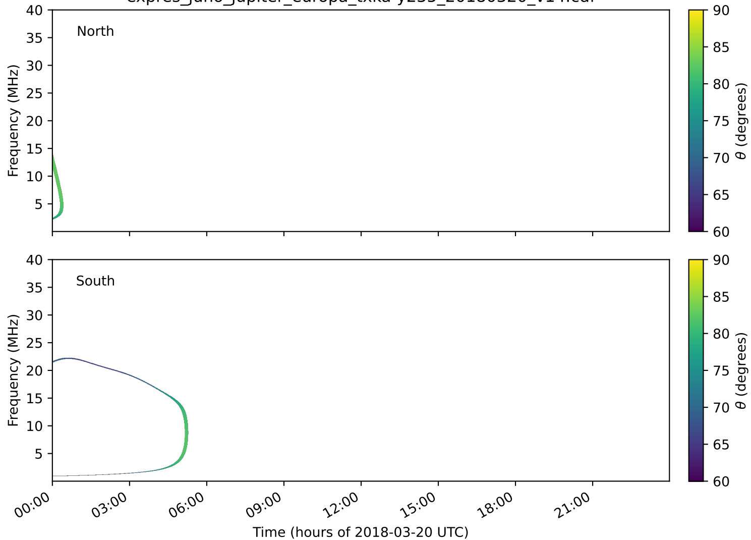
expres_juno_jupiter_europa_txka-y235_20180320_v14.cdf
