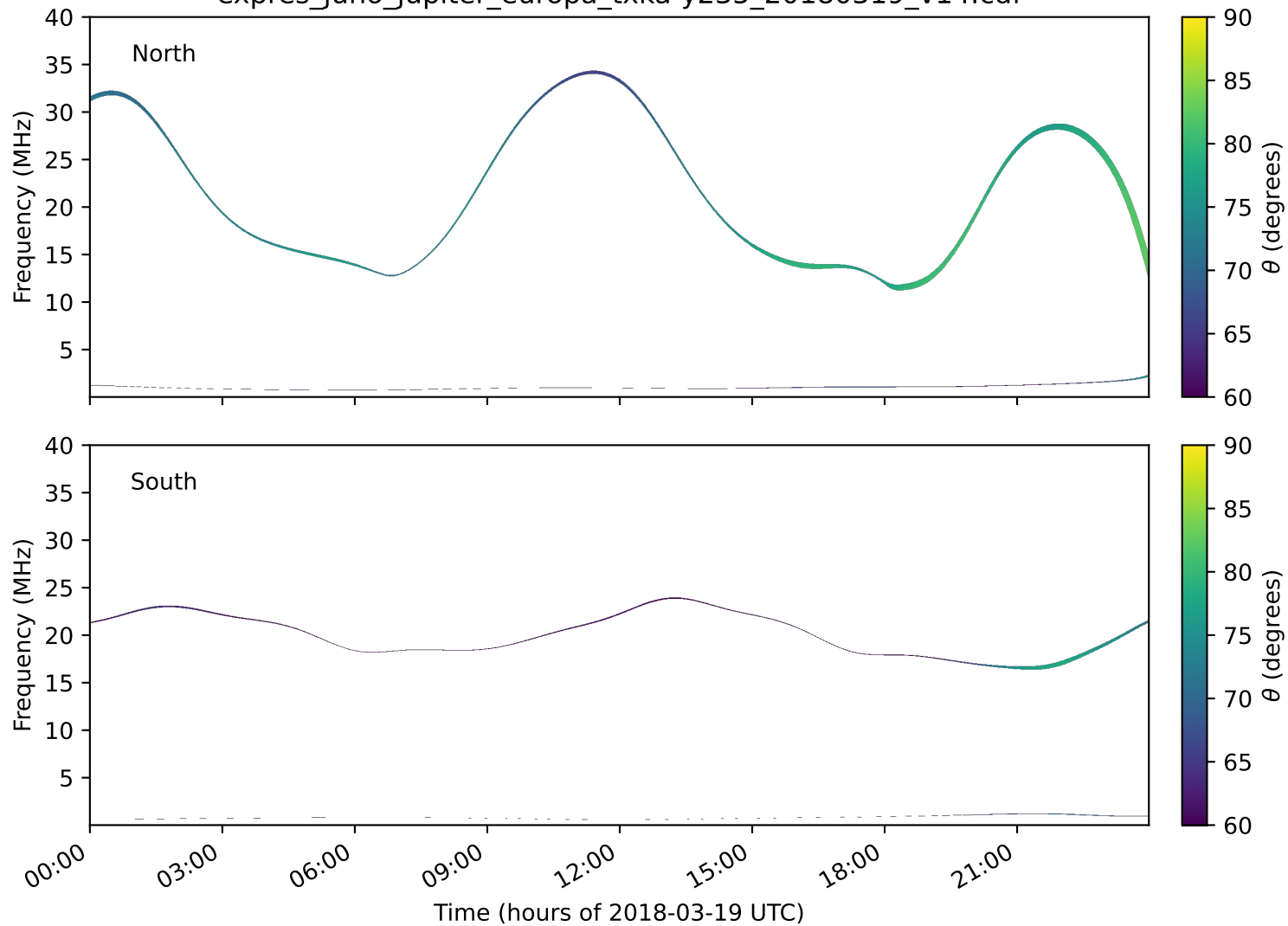
expres_juno_jupiter_europa_txka-y235_20180319_v14.cdf
