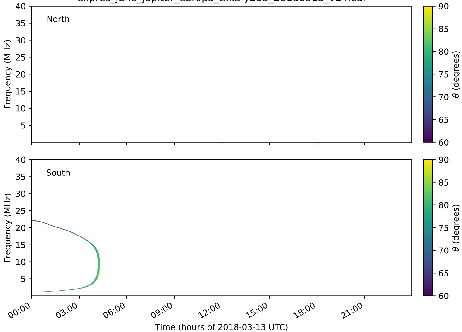
expres_juno_jupiter_europa_txka-y235_20180313_v14.cdf
