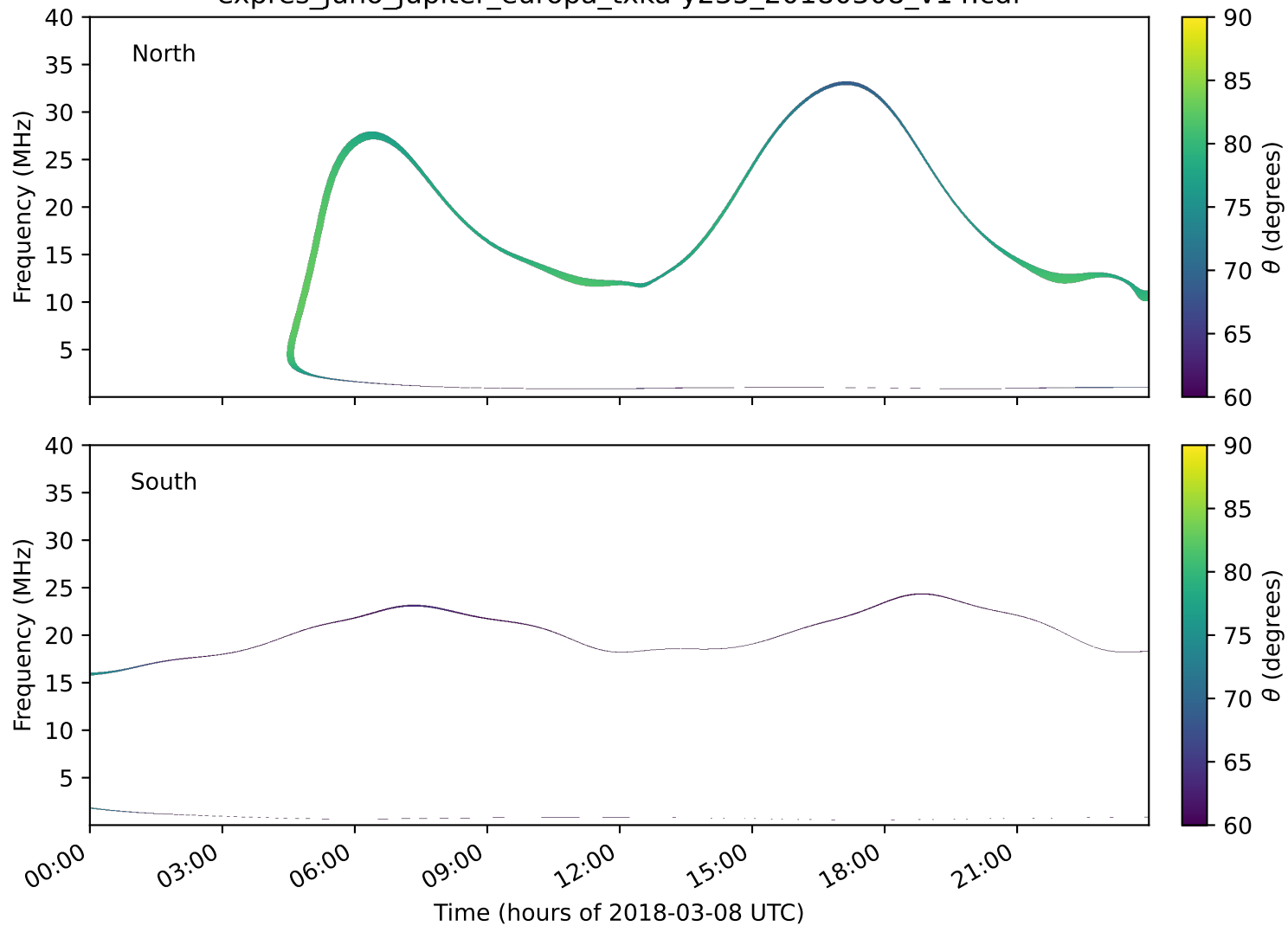
expres_juno_jupiter_europa_txka-y235_20180308_v14.cdf
