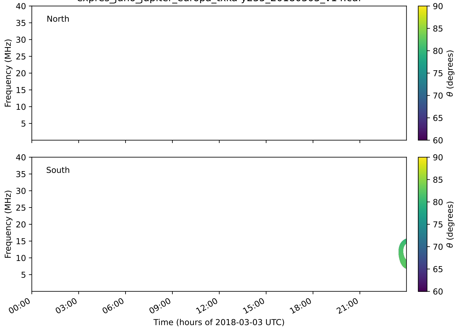
expres_juno_jupiter_europa_txka-y235_20180303_v14.cdf
