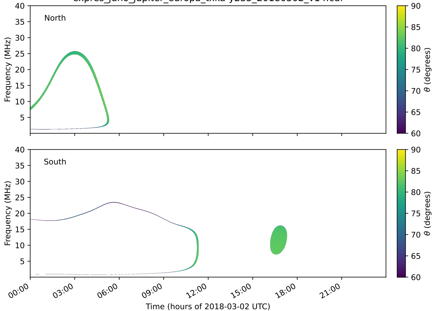
expres_juno_jupiter_europa_txka-y235_20180302_v14.cdf
