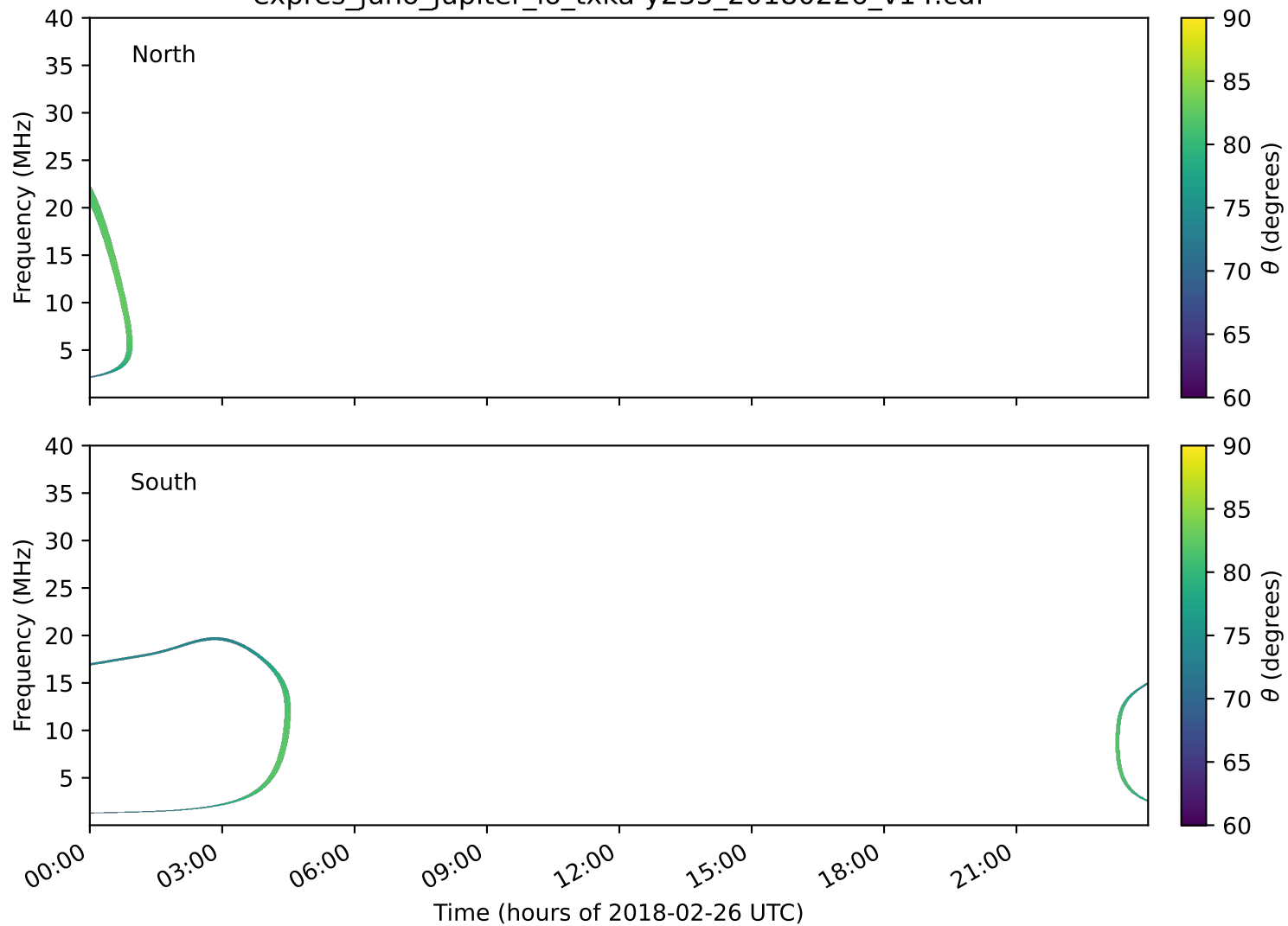
expres_juno_jupiter_io_txka-y235_20180226_v14.cdf
