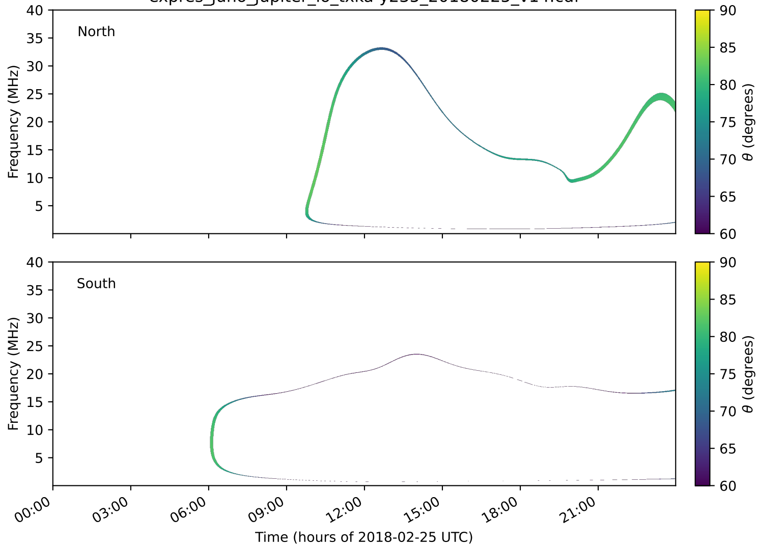
expres_juno_jupiter_io_txka-y235_20180225_v14.cdf
