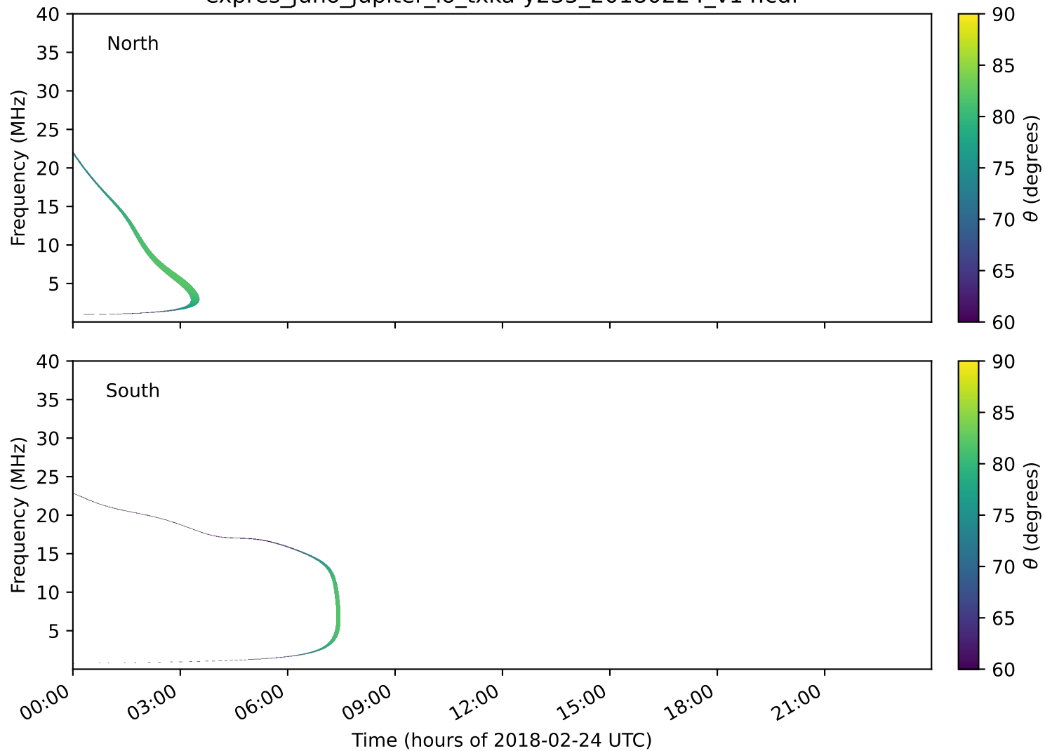
expres_juno_jupiter_io_txka-y235_20180224_v14.cdf
