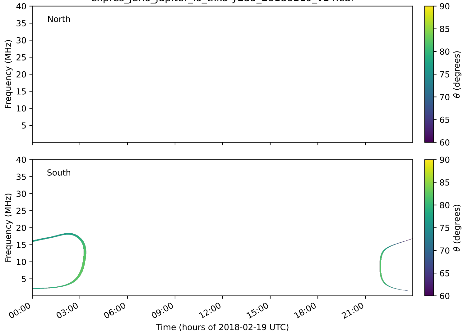
expres_juno_jupiter_io_txka-y235_20180219_v14.cdf
