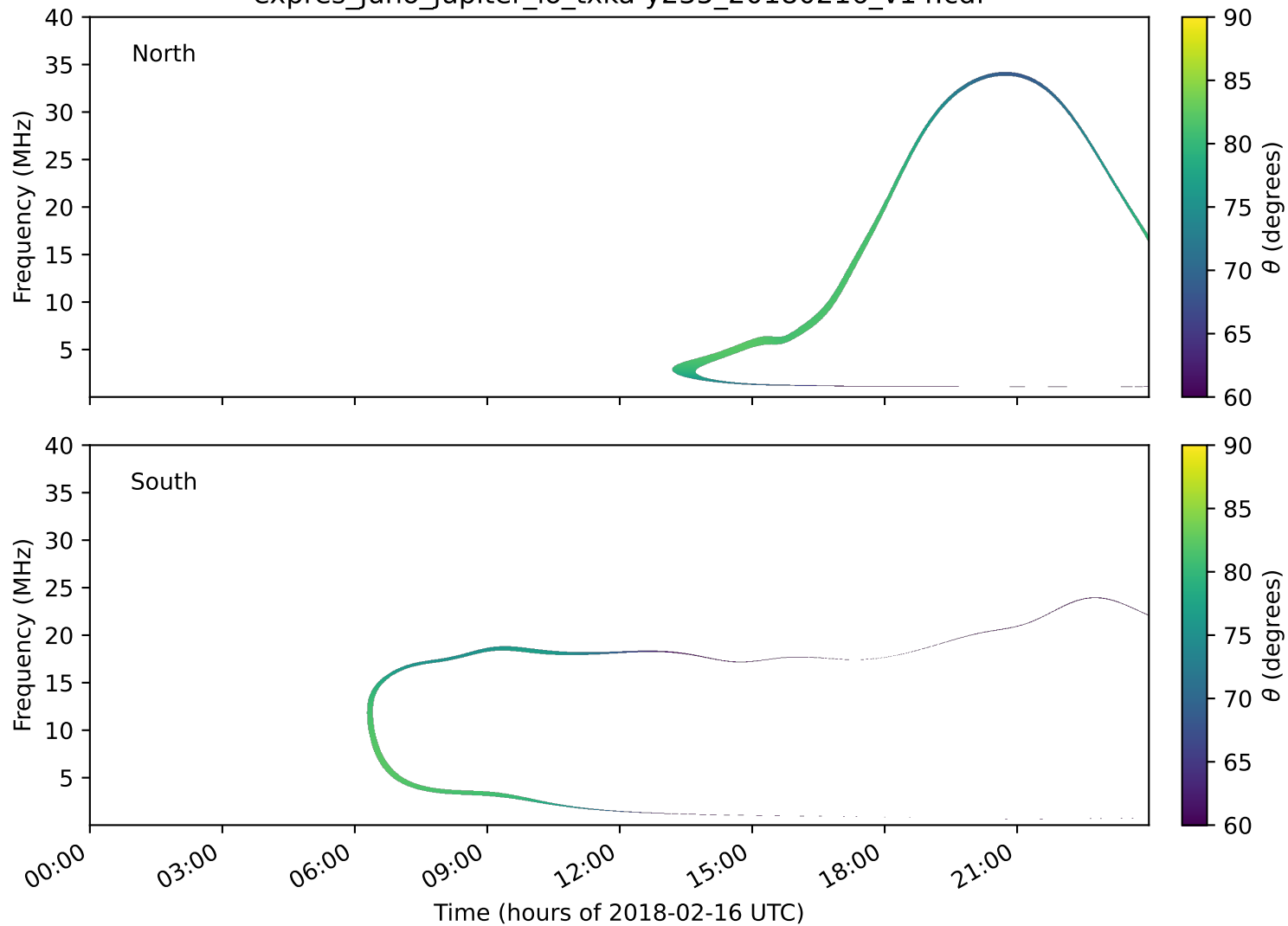
expres_juno_jupiter_io_txka-y235_20180216_v14.cdf
