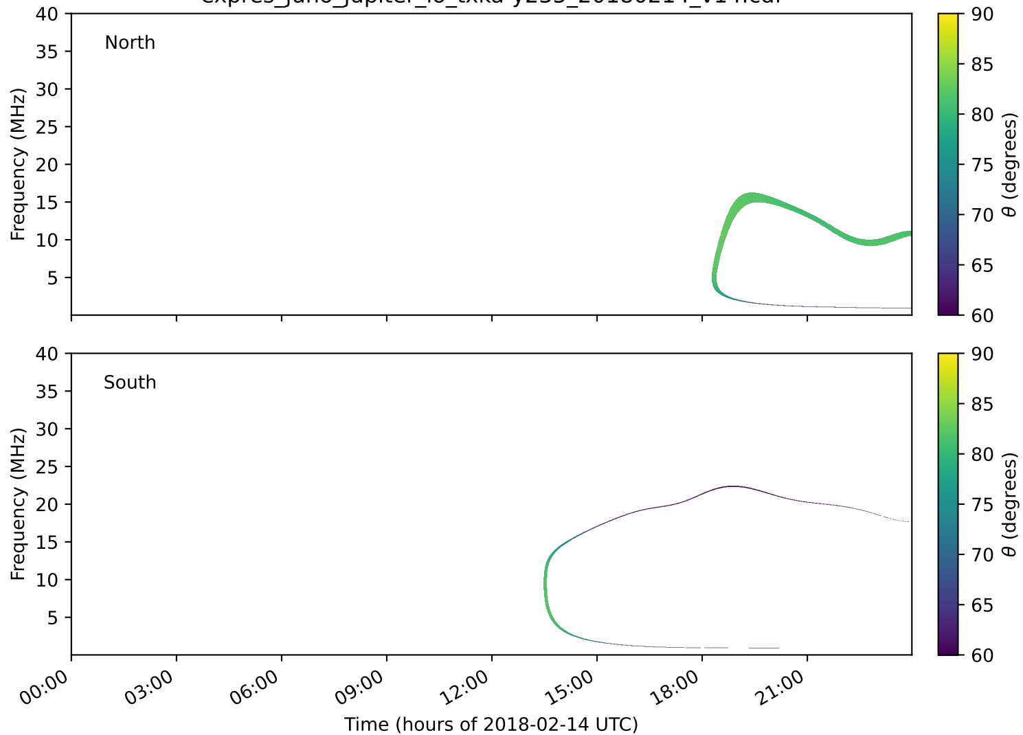
expres_juno_jupiter_io_txka-y235_20180214_v14.cdf
