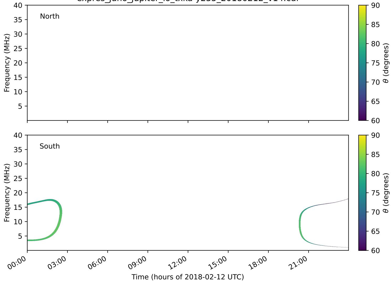
expres_juno_jupiter_io_txka-y235_20180212_v14.cdf
