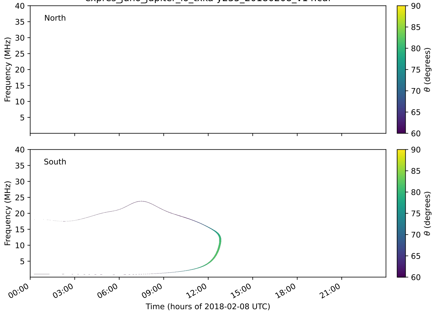
expres_juno_jupiter_io_txka-y235_20180208_v14.cdf
