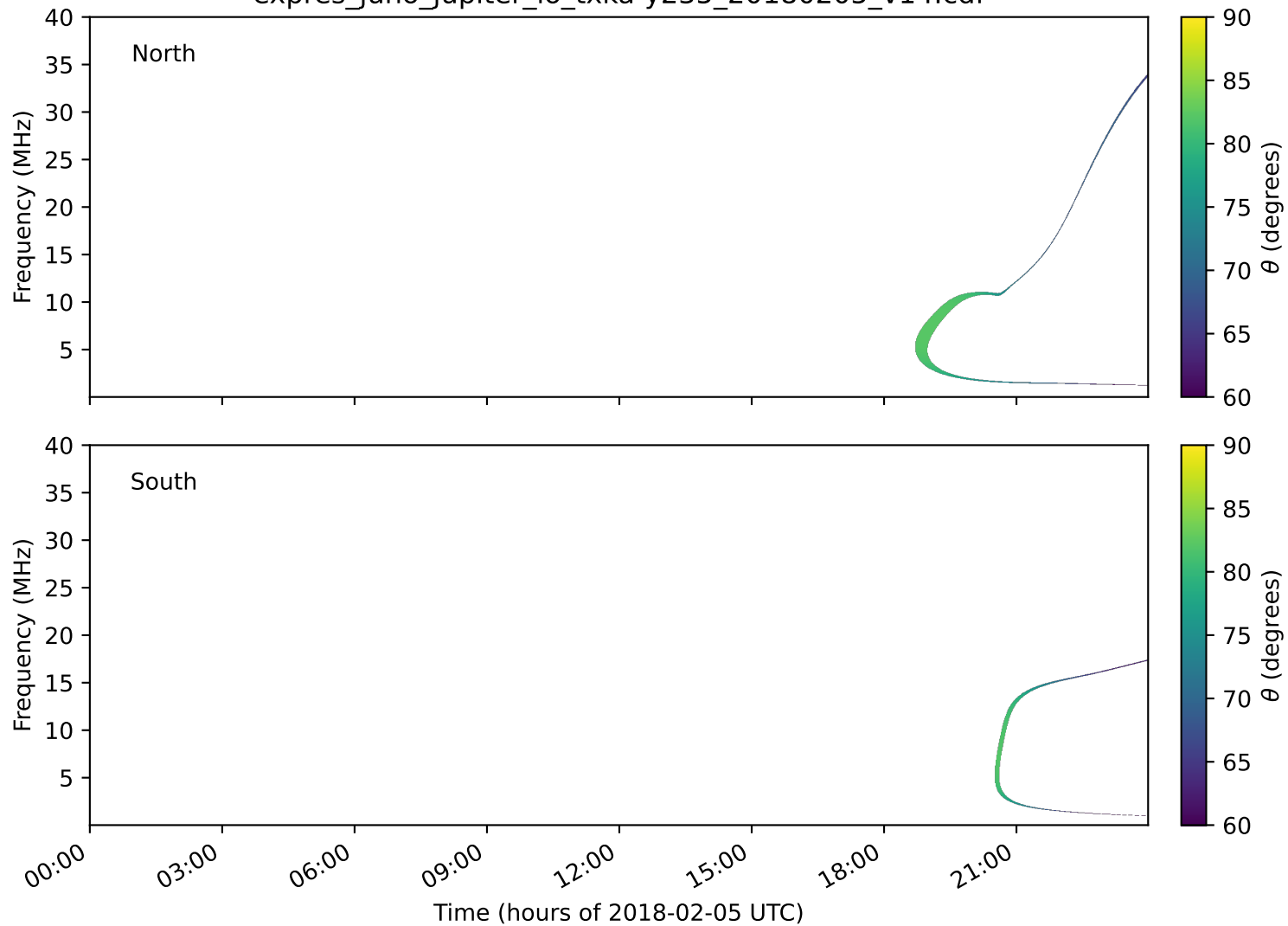
expres_juno_jupiter_io_txka-y235_20180205_v14.cdf
