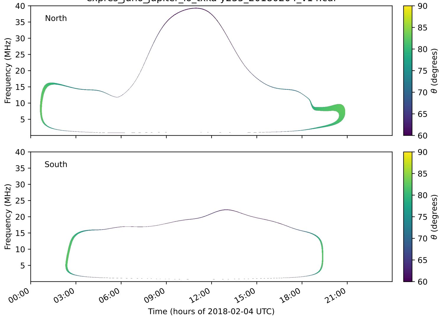
expres_juno_jupiter_io_txka-y235_20180204_v14.cdf
