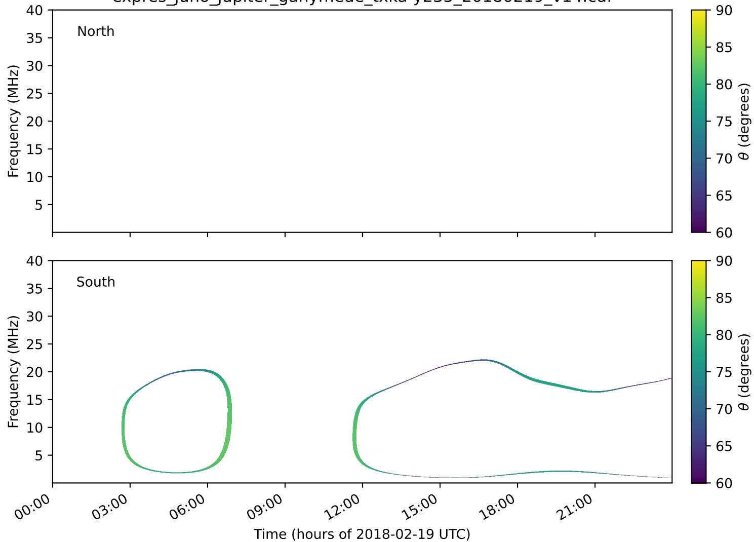
expres_juno_jupiter_ganymede_txka-y235_20180219_v14.cdf
