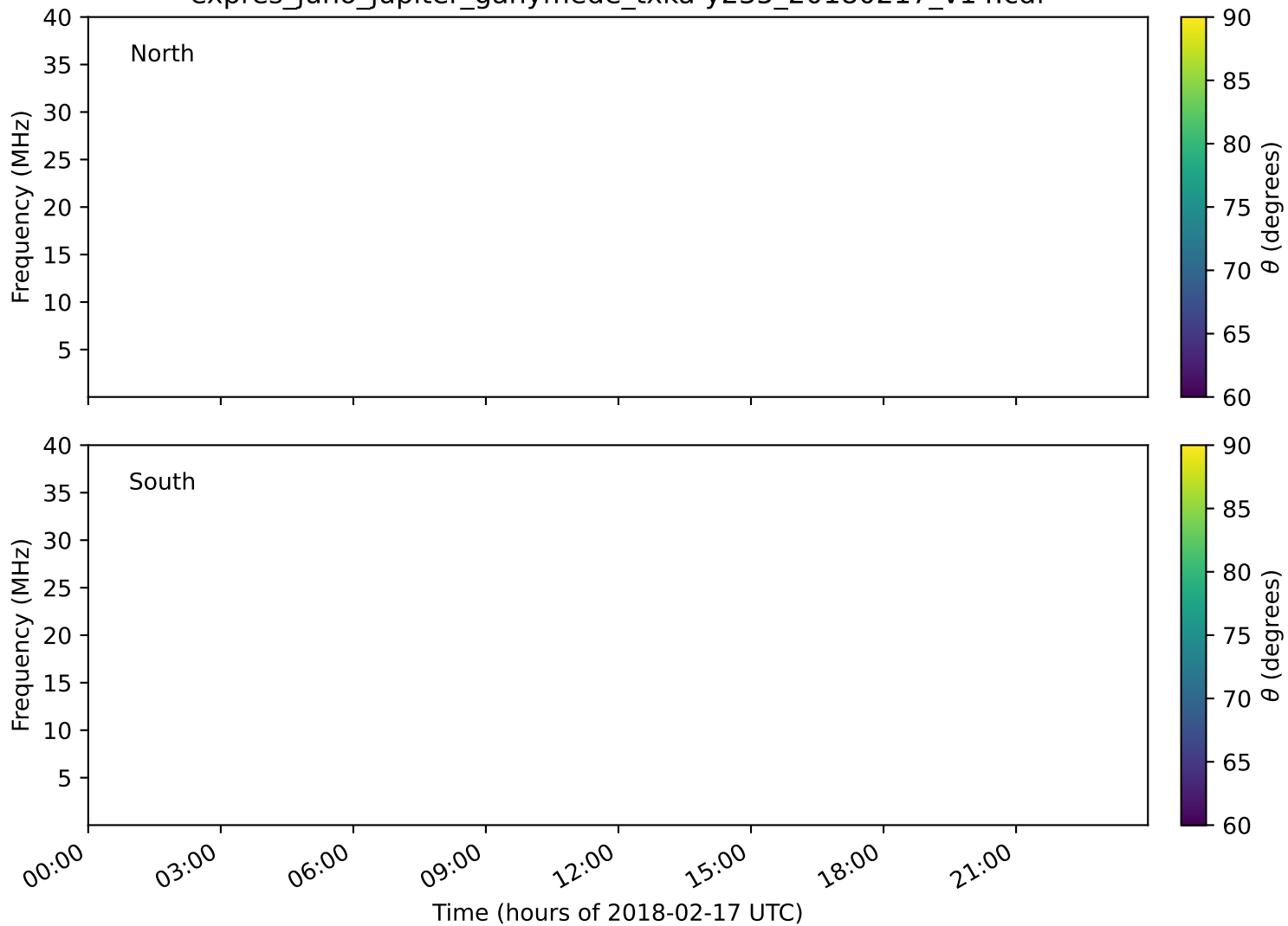
expres_juno_jupiter_ganymede_txka-y235_20180217_v14.cdf
