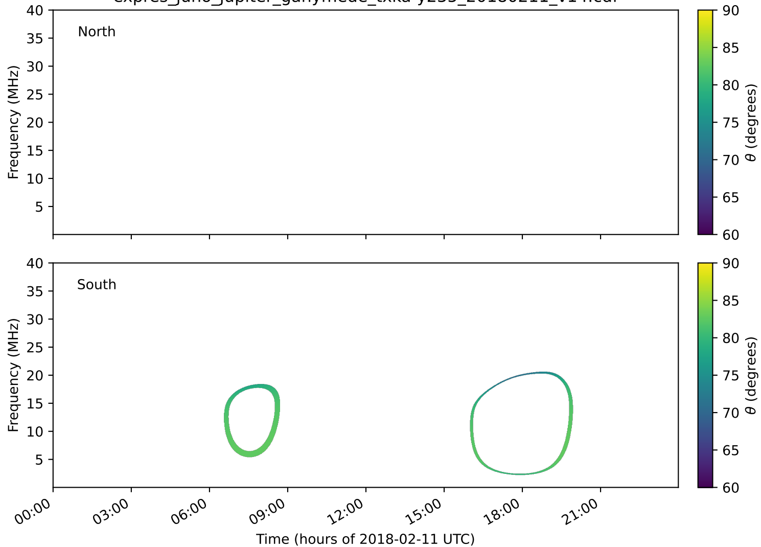
expres_juno_jupiter_ganymede_txka-y235_20180211_v14.cdf
