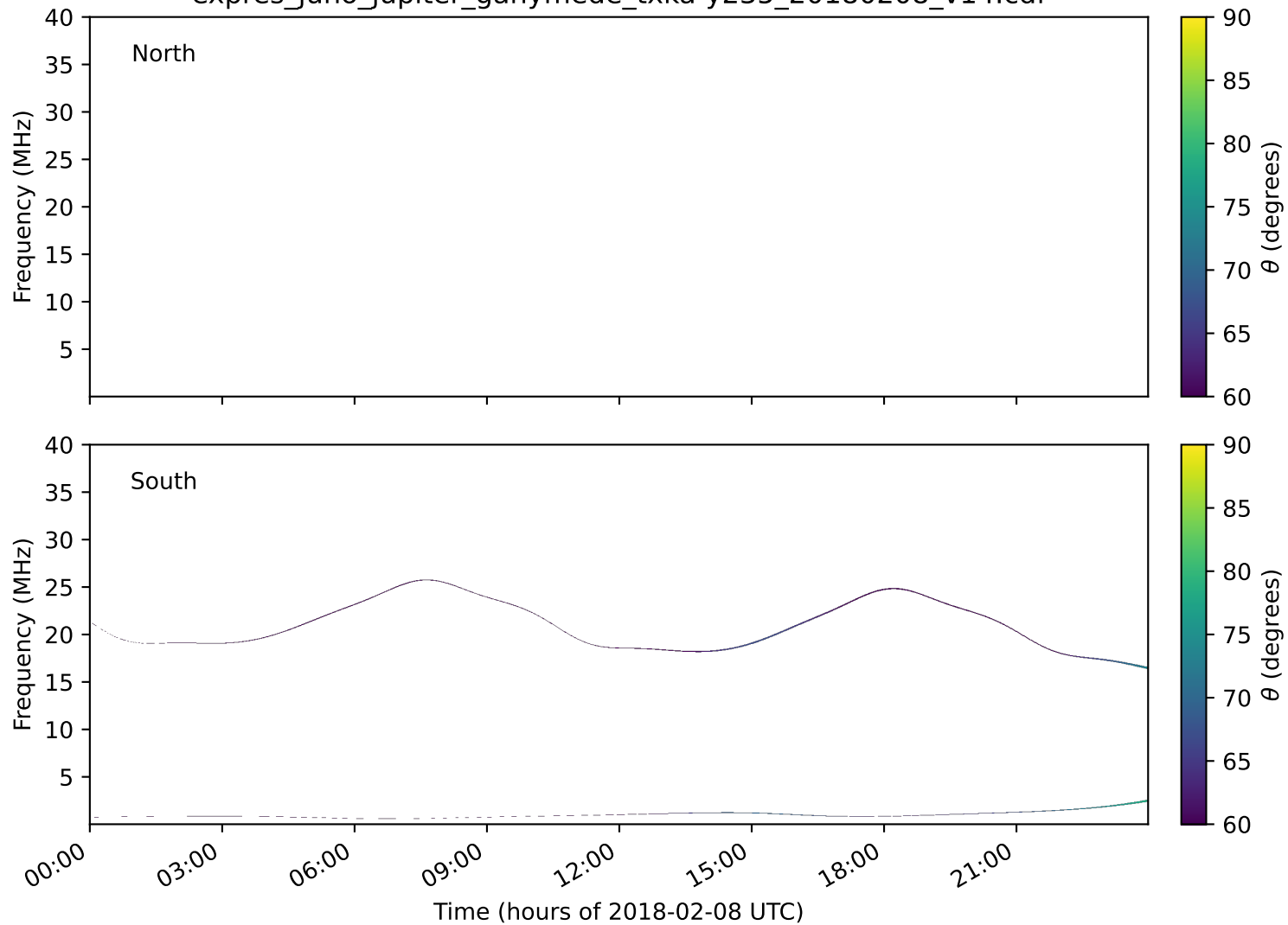
expres_juno_jupiter_ganymede_txka-y235_20180208_v14.cdf
