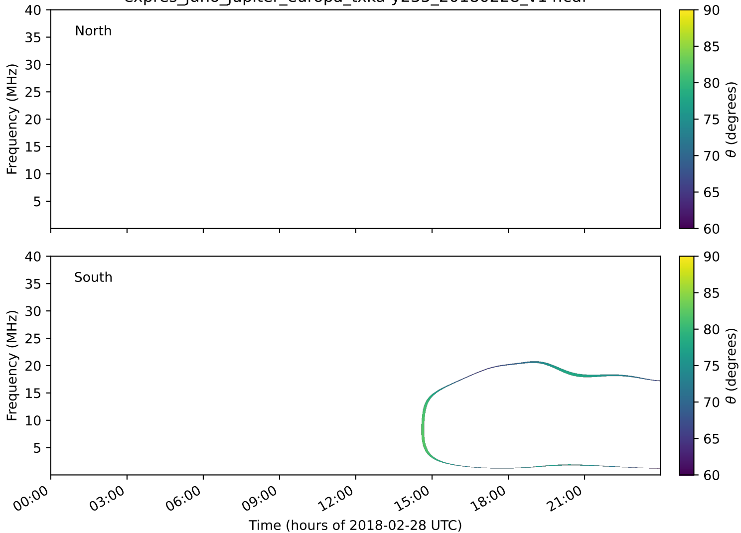
expres_juno_jupiter_europa_txka-y235_20180228_v14.cdf
