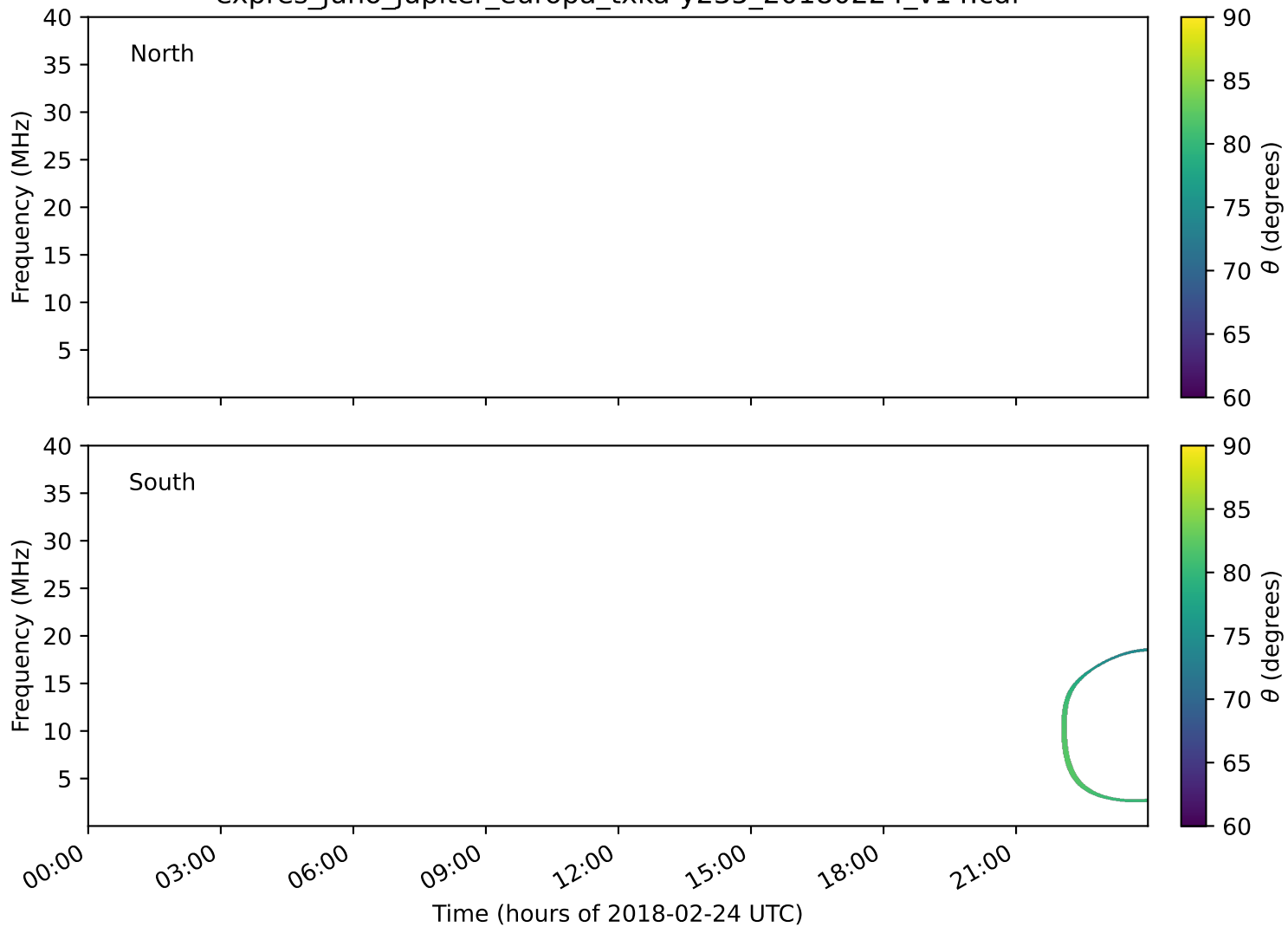
expres_juno_jupiter_europa_txka-y235_20180224_v14.cdf
