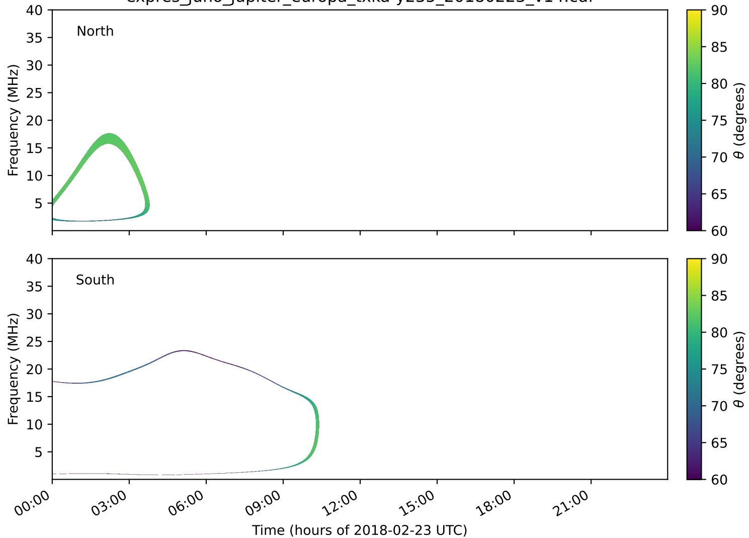
expres_juno_jupiter_europa_txka-y235_20180223_v14.cdf
