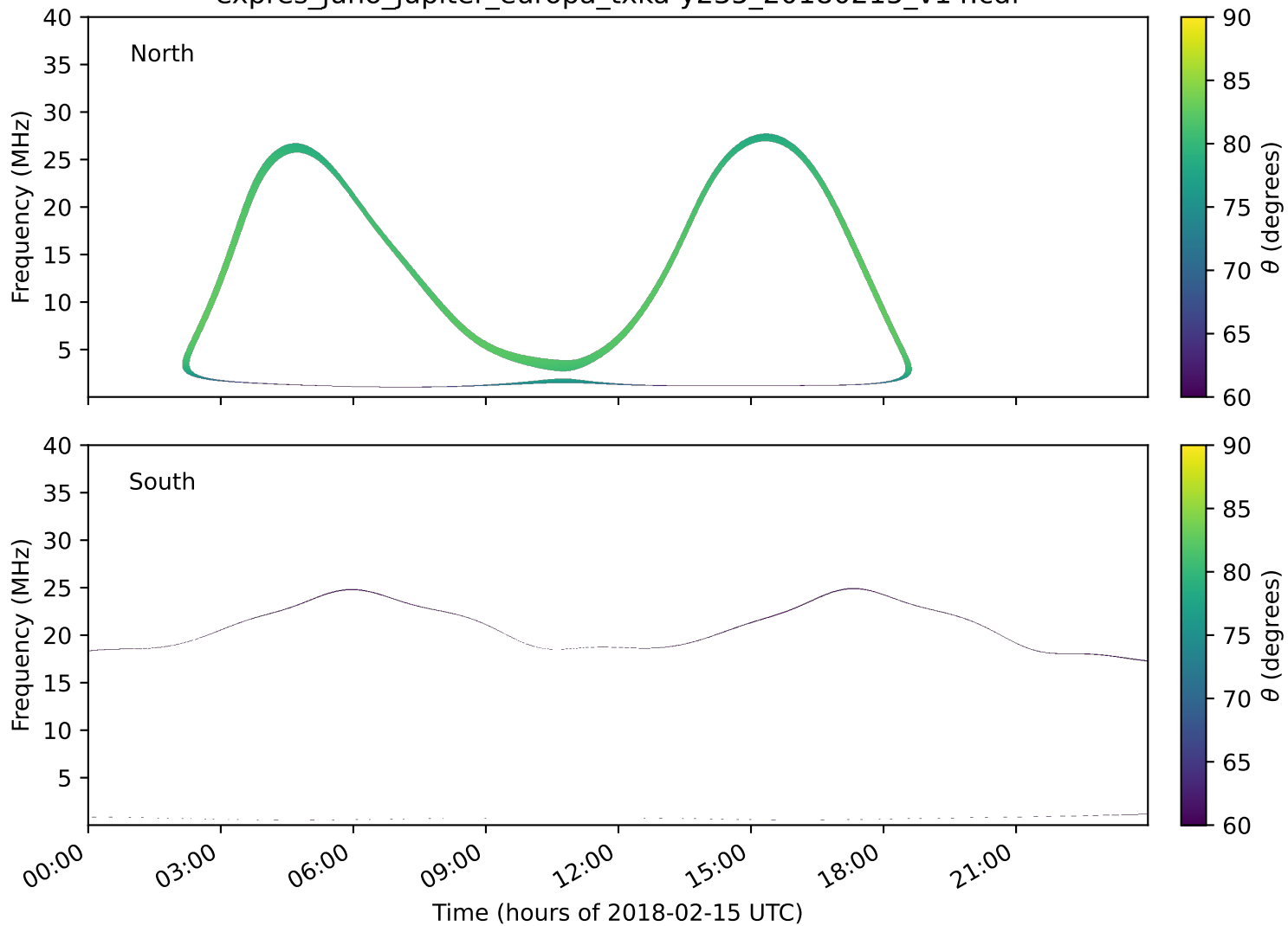
expres_juno_jupiter_europa_txka-y235_20180215_v14.cdf
