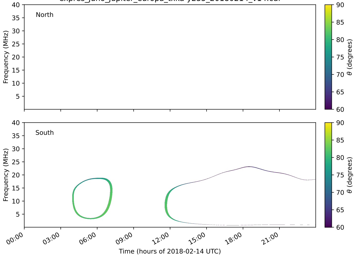
expres_juno_jupiter_europa_txka-y235_20180214_v14.cdf
