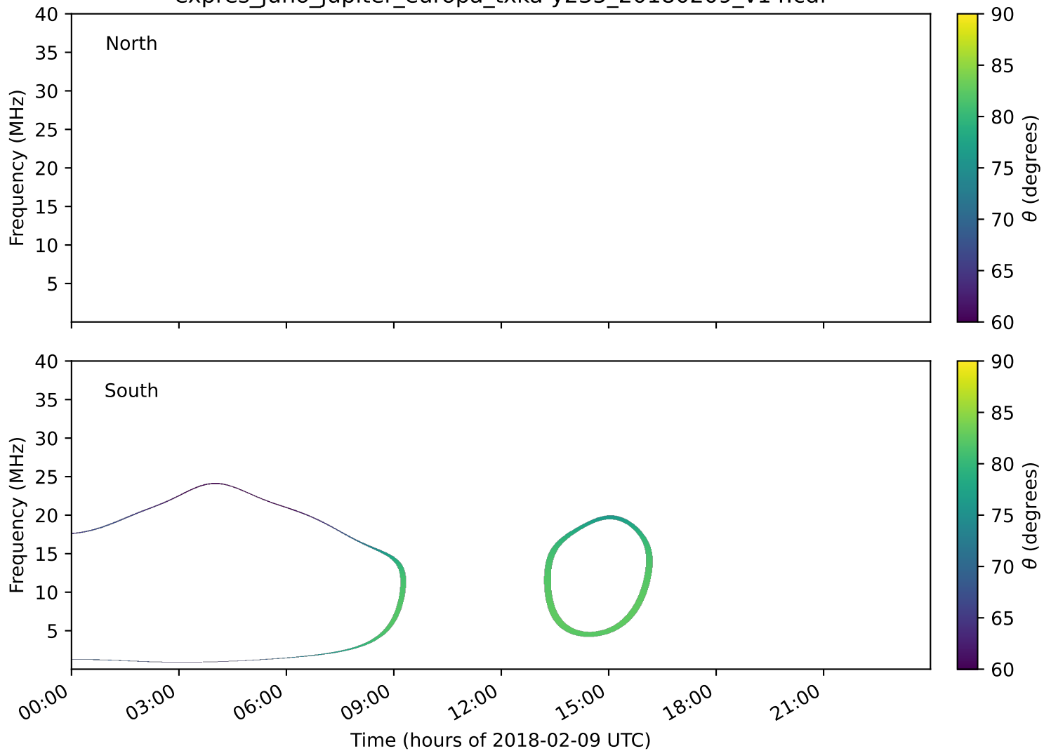
expres_juno_jupiter_europa_txka-y235_20180209_v14.cdf
