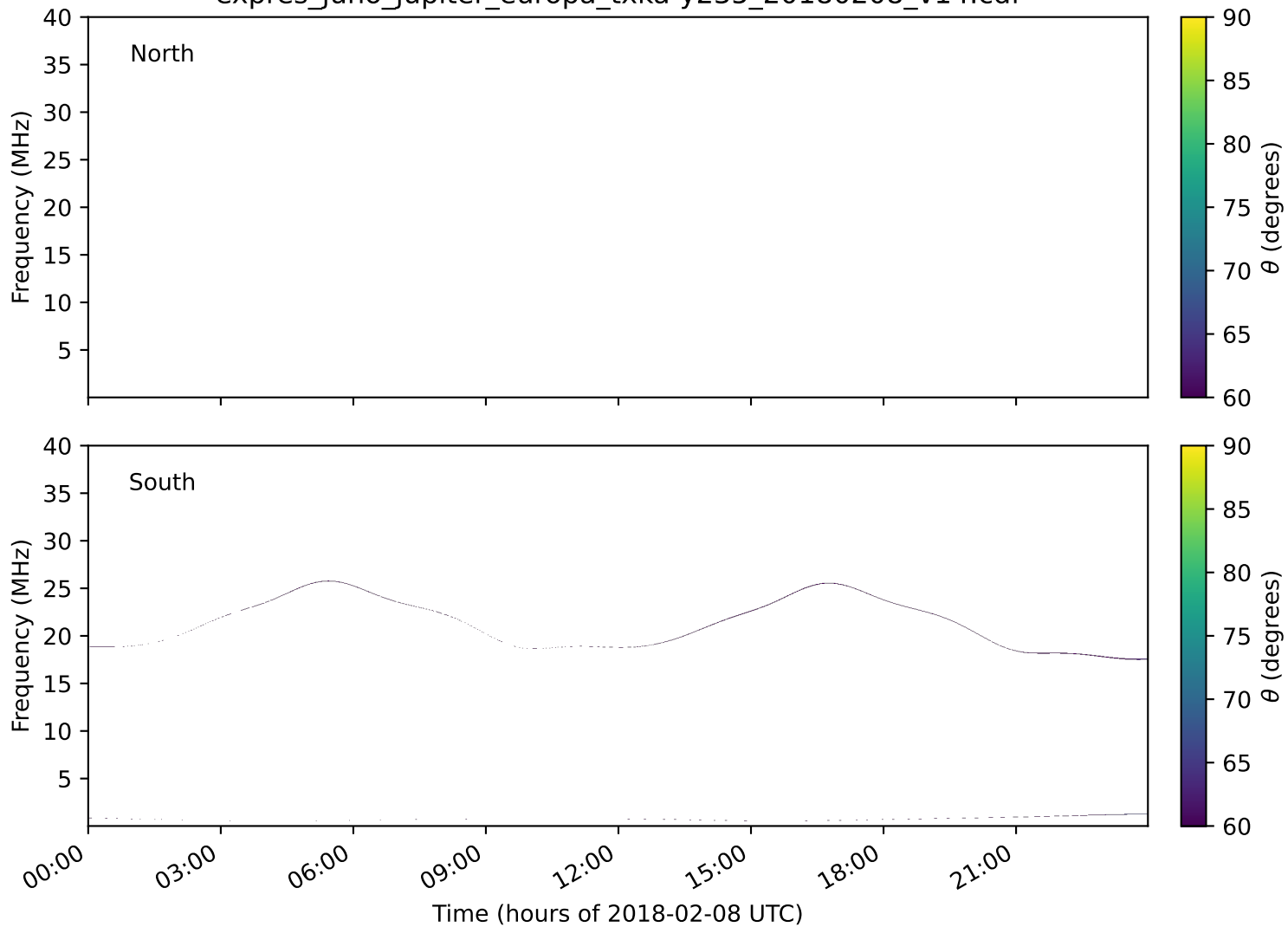
expres_juno_jupiter_europa_txka-y235_20180208_v14.cdf
