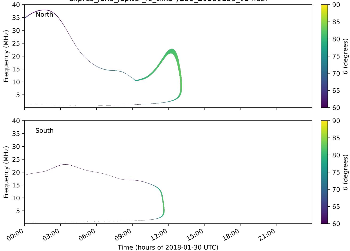
expres_juno_jupiter_io_txka-y235_20180130_v14.cdf
