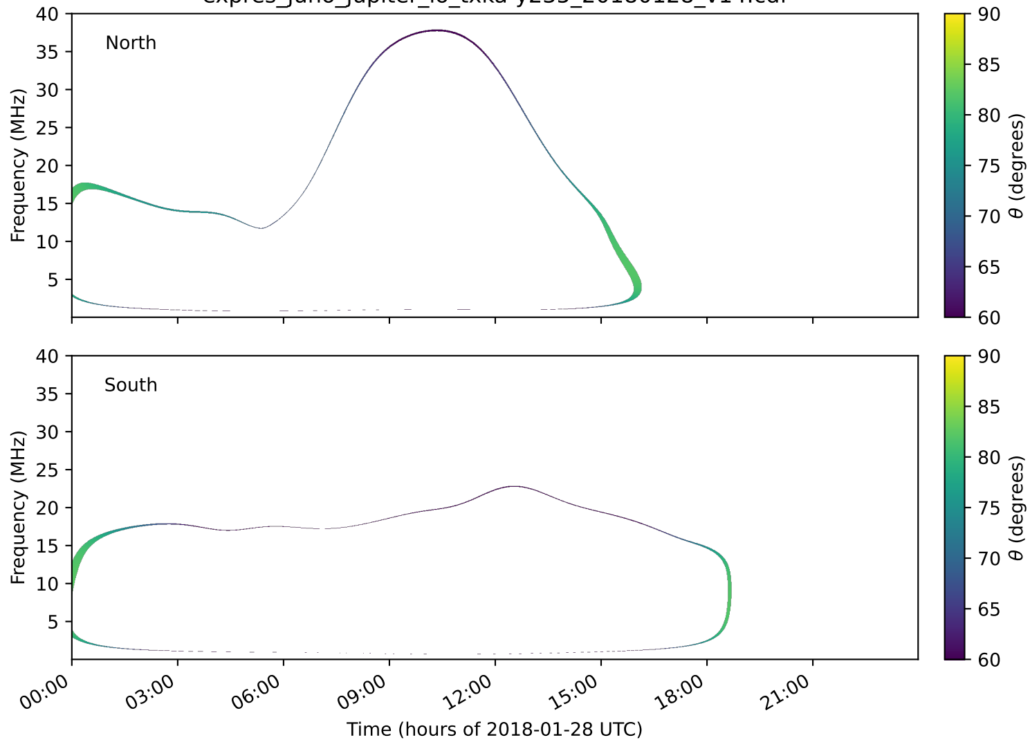
expres_juno_jupiter_io_txka-y235_20180128_v14.cdf
