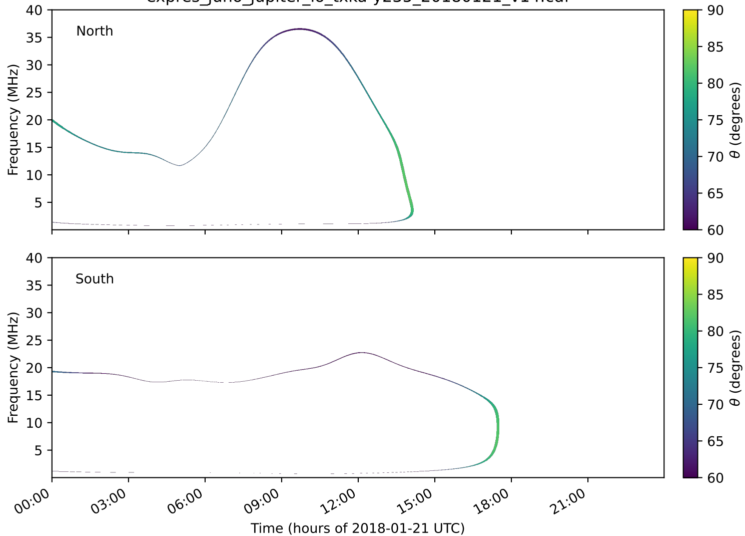
expres_juno_jupiter_io_txka-y235_20180121_v14.cdf
