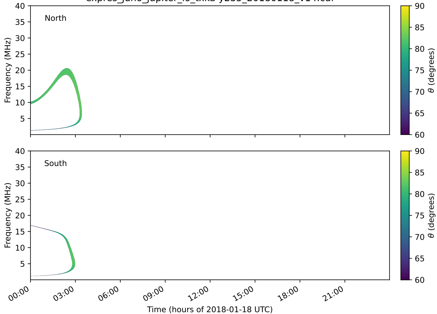
expres_juno_jupiter_io_txka-y235_20180118_v14.cdf
